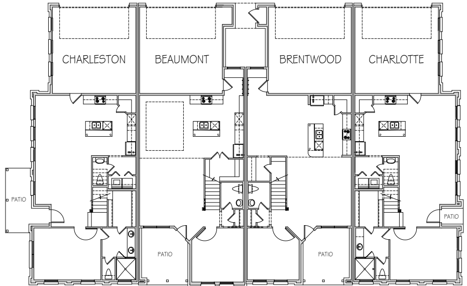
FIRST FLOOR PARKLAND BUILDING PLAN
