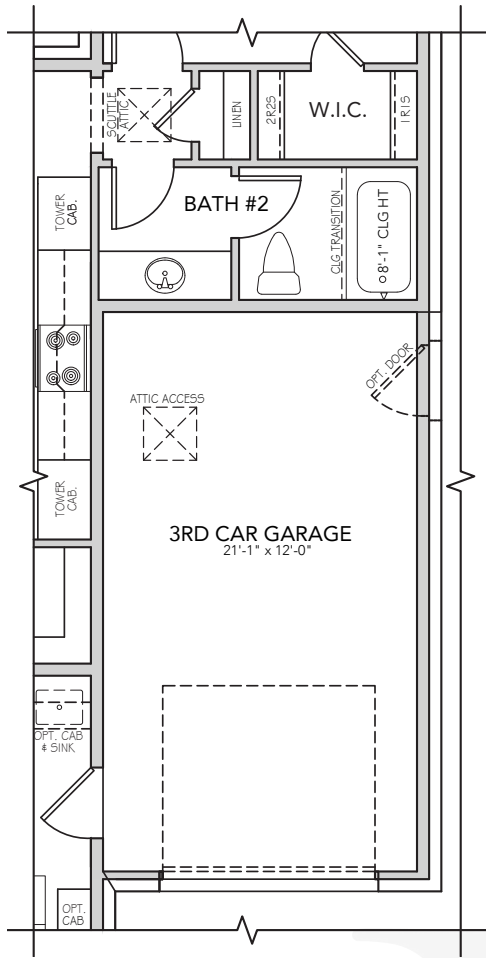
OPT. 3RD CAR GARAGE
