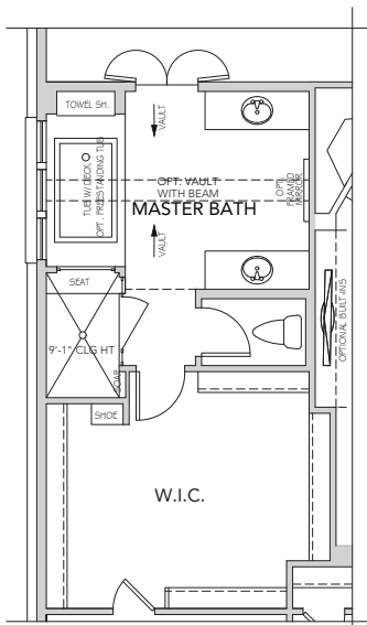
OPT. MASTER BATH LAYOUT
