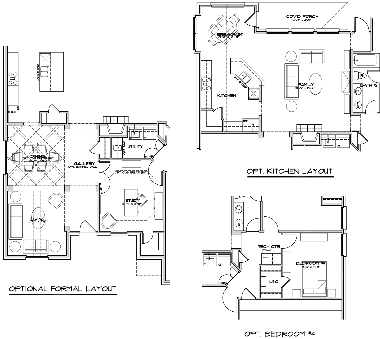
BRAXTON II FIRST FLOOR PLAN OPTIONS
